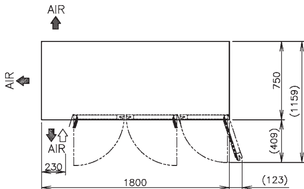
VIEW A(1/10)
